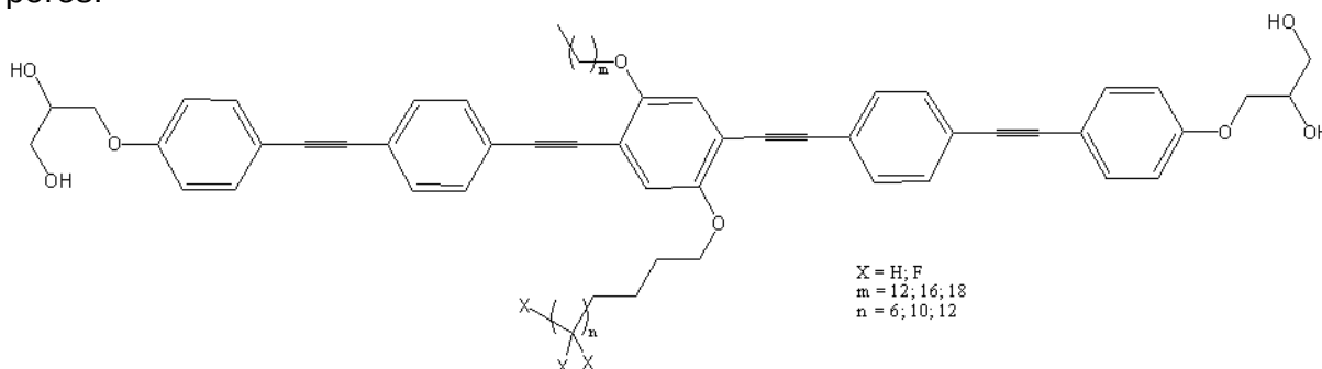
Fig. 1: Chemical structure of polyphilic molecules used in this study
