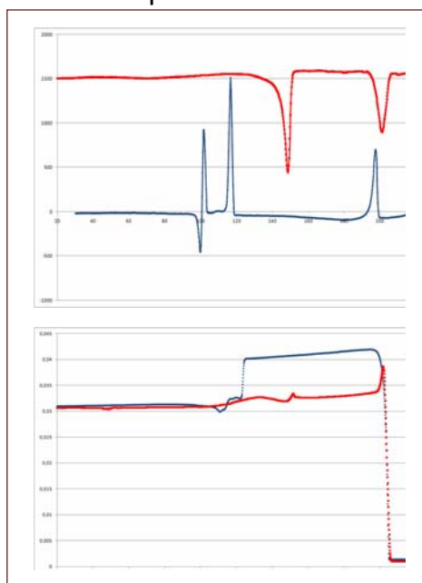
Fig.1. Thermo-optic (TOA) and calorimetric (DSC) characteristics of decyl derivative.
