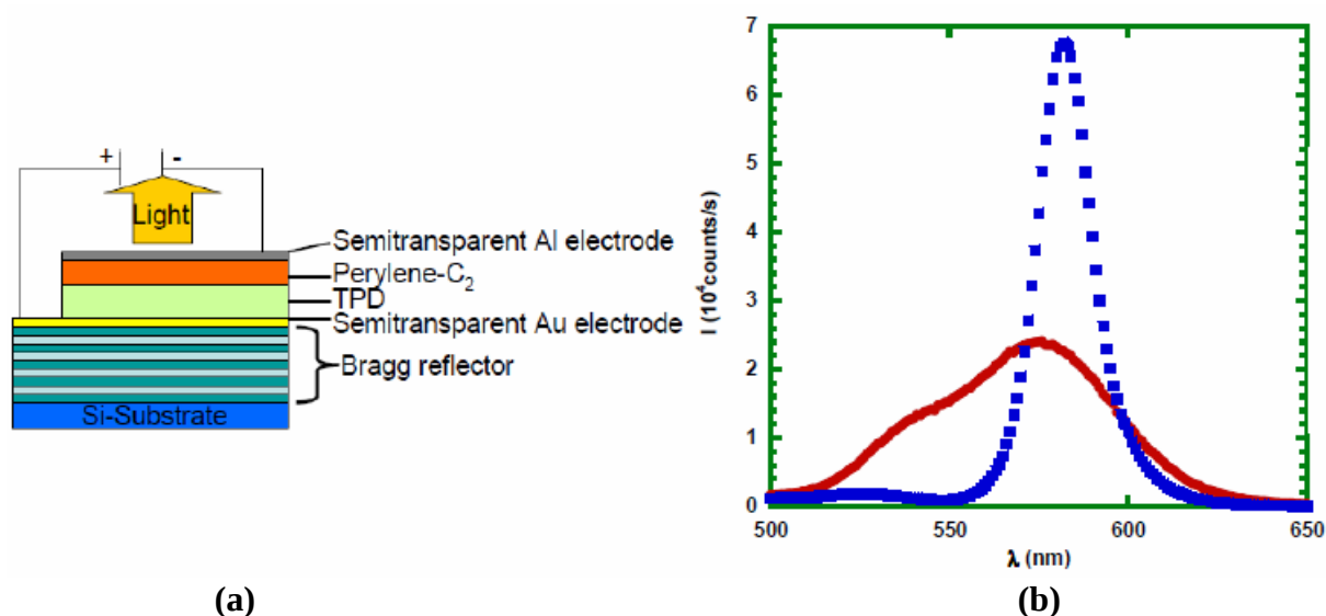
Figure 1: (a) Schematic structure of the OLEDs. (b) Electroluminescence spectrum of a reference sample on ITO-coated glass without Bragg reflector (red) and a cavity enhanced sample (blue).
