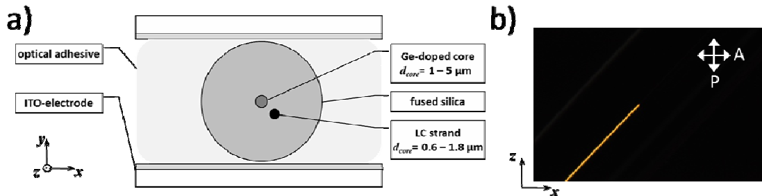
Fig.1. Scheme of a step-index fiber with an air hole liquid-crystal-filled channel, glued between two planar ITO-electrodes ( \approx 200 nm electrode gap). b) Transmitted light polarized optical micrograph (crossed polarizers) of a fiber with one single hollow channel (1.8 \mu\text{m} diameter). A 7 cm length is filled with E7. The end of the LC-strand is shown in order to distinguish the LC-filled section from the silica glass background.
