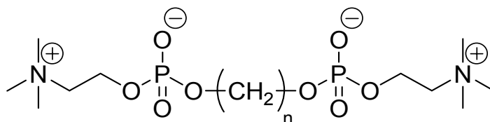
Figure 1: Chemical structure of PC-Cn-PC with n=22-32
