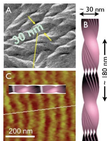
Figure: A) TEM image of B4 nano-rods showing exposed layer edges. B) Illustration of the structure of the rods. C) AFM image of aligned B4 indicating orientation of the rods (not to scale).
