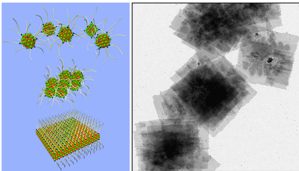
(left) Scheme of individual nanocrystals merging into a two dimensional structure. (right) Electron-microscopy image of synthesized lead sulfide sheets with a lateral dimensions in the micrometer range and a height of about two nanometers.
